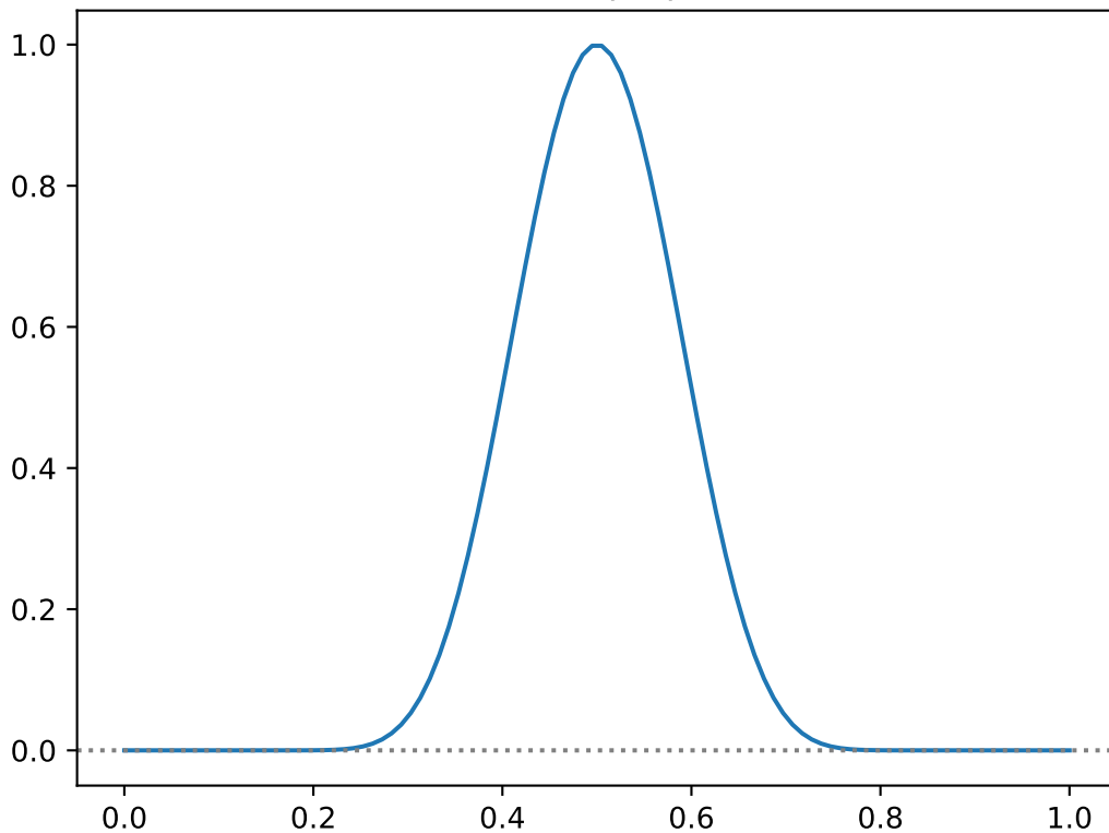
Gauss bump: q=4.00
